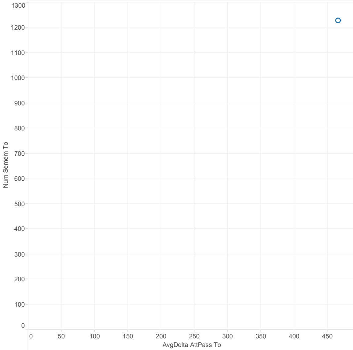
Sum of AvgDelta AttPass To and sum of AvgQualPts To vs. sum of Num Semem To.
